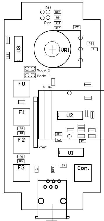
View from Surface mount side
